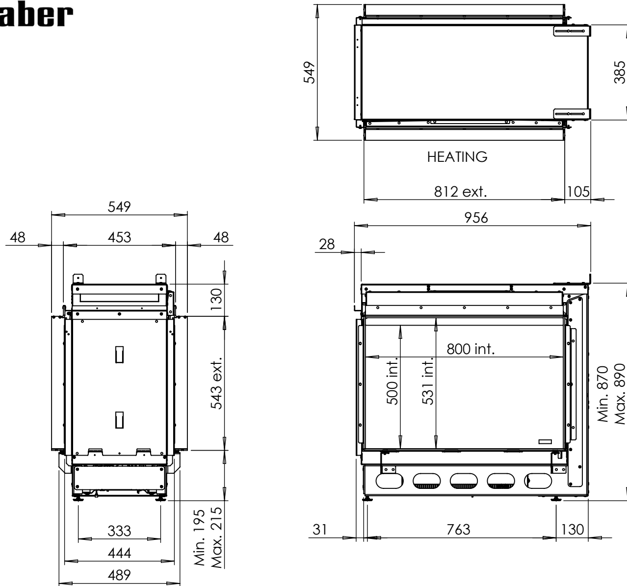
Dimensional Drawing e-Matrix heat 800x500 ST (MkII)
