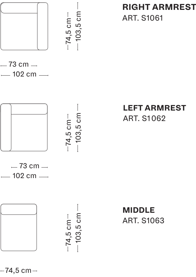
MAGS SOFT NARROW MODULE
