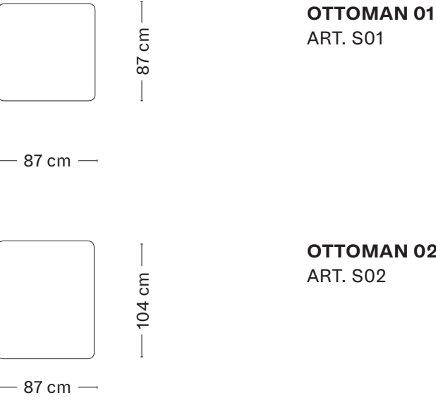
MAGS SOFT OTTOMAN
