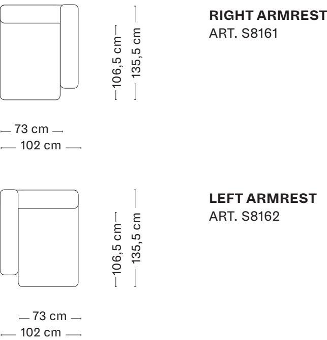
MAGS SOFT NARROW CHAISE LONGUE MODULE SHORT
