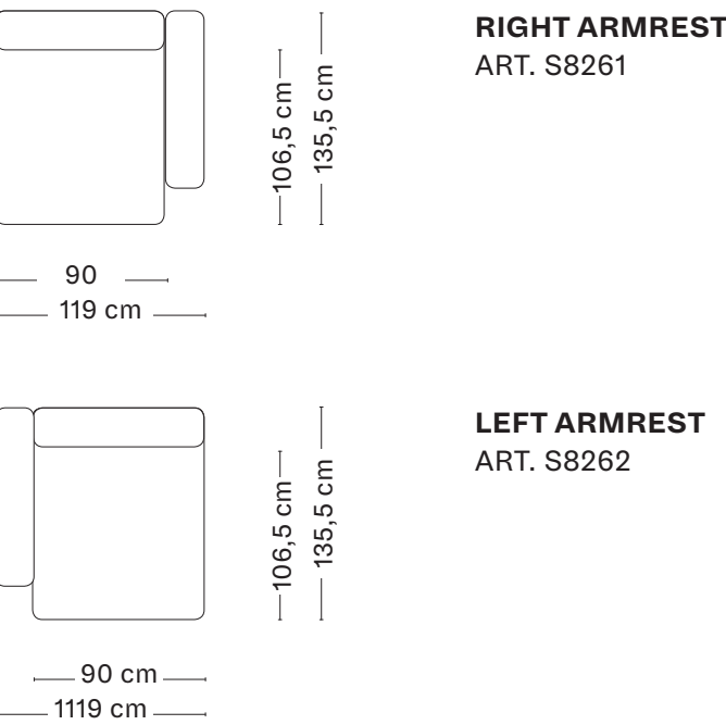
MAGS SOFT WIDE CHAISE LONGUE MODULE SHORT
