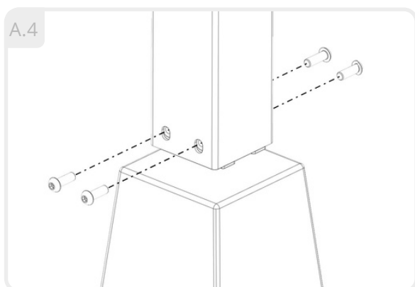
A.4 Use the supplied bolts to fix the support to the base plate.
