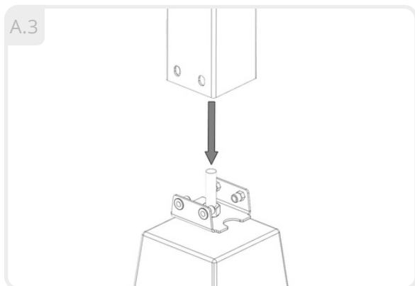
A.3 Slide the support over the base plate; ensure the screw holes on both parts face the same direction.
