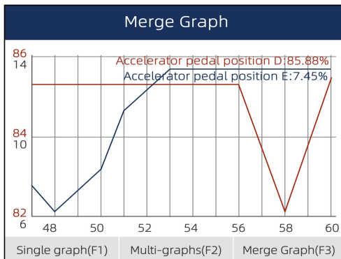
Figure 5-14 Sample Merged PID Plots Screen
