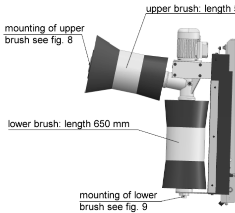
Figure 7: Overview of brush replacement
