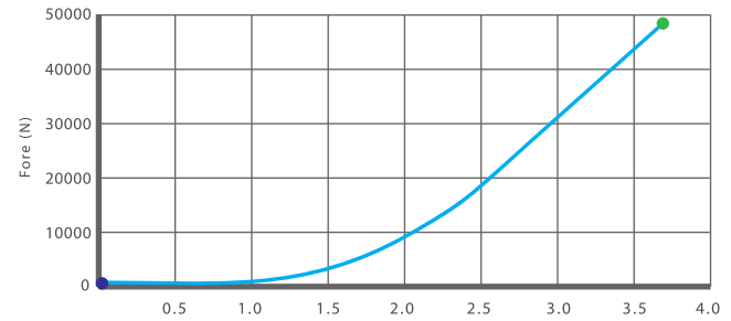
COMPRESSION TEST (COLD -40°)
