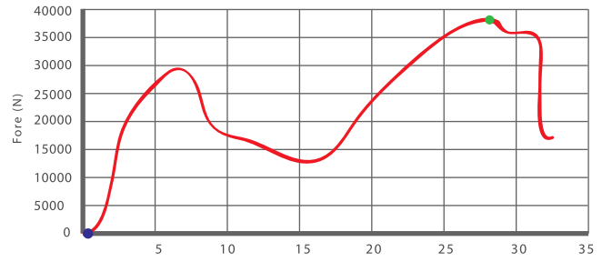
COMPRESSION TEST (HOT 23°)
