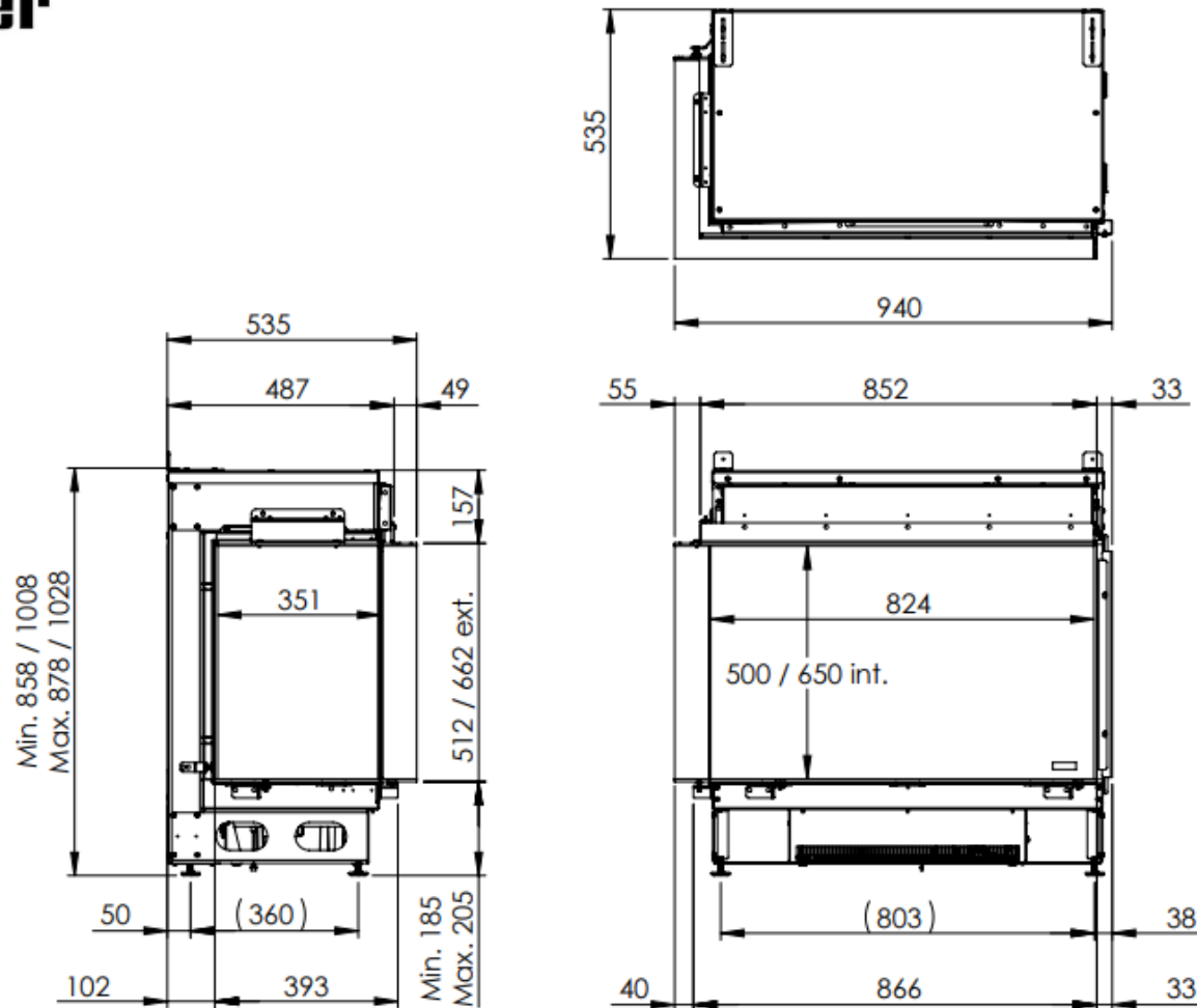
Dimensional Drawing e-MatriX 800/500 IIL + 800/650 IIL (MkII)
