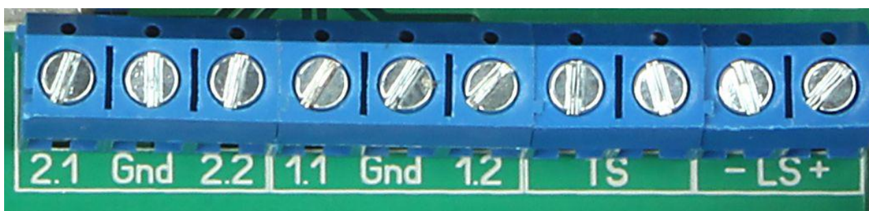
Illustration 1: Terminal strip PHB
