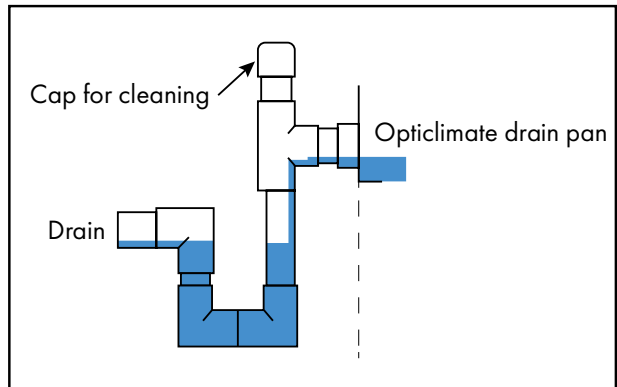
Correct drain installation
