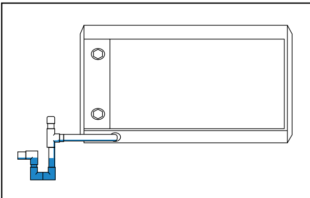
Condensation drain connection
