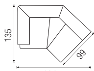
194 45 corner small arm L top view
