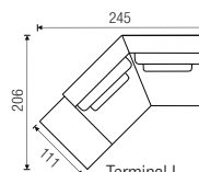
Terminal L top view
