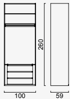
D 02 Double Cabinet CABINET WITH DRAWERS
