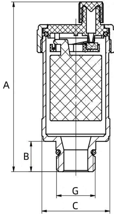
Automatic air vent valve 1/2" with automatic shut-off Working temperature: Max. 110°C Working pressure: 10 bar
