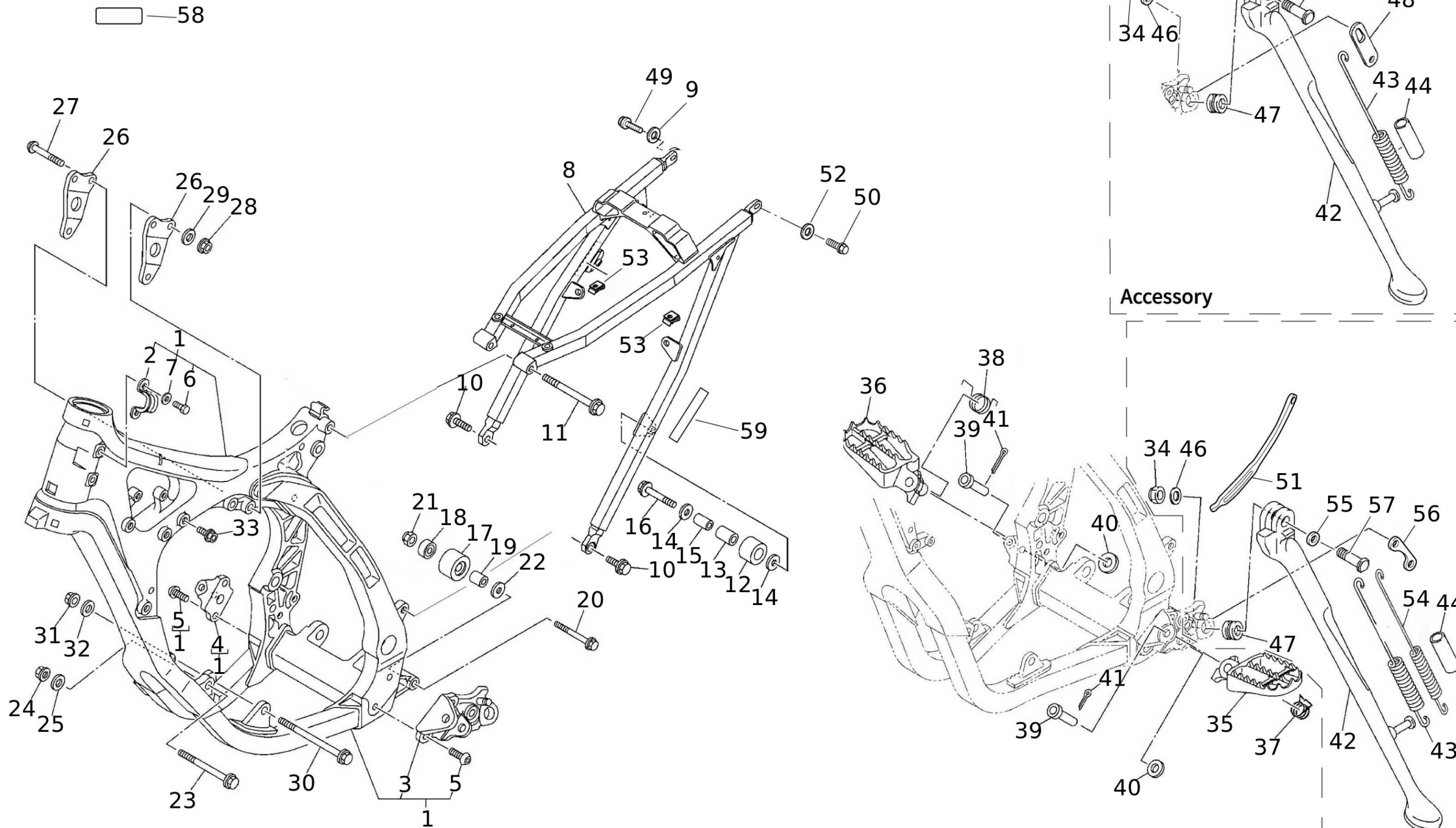
1 - Frame / Footpegs / Stand (XE 125 MY23)
