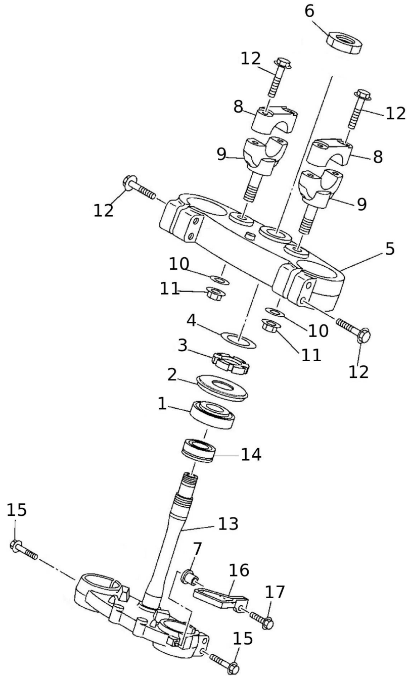
4 - Steering plates
