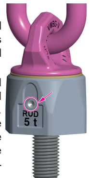
Pic. 6: Funnel-shaped grease nipple
