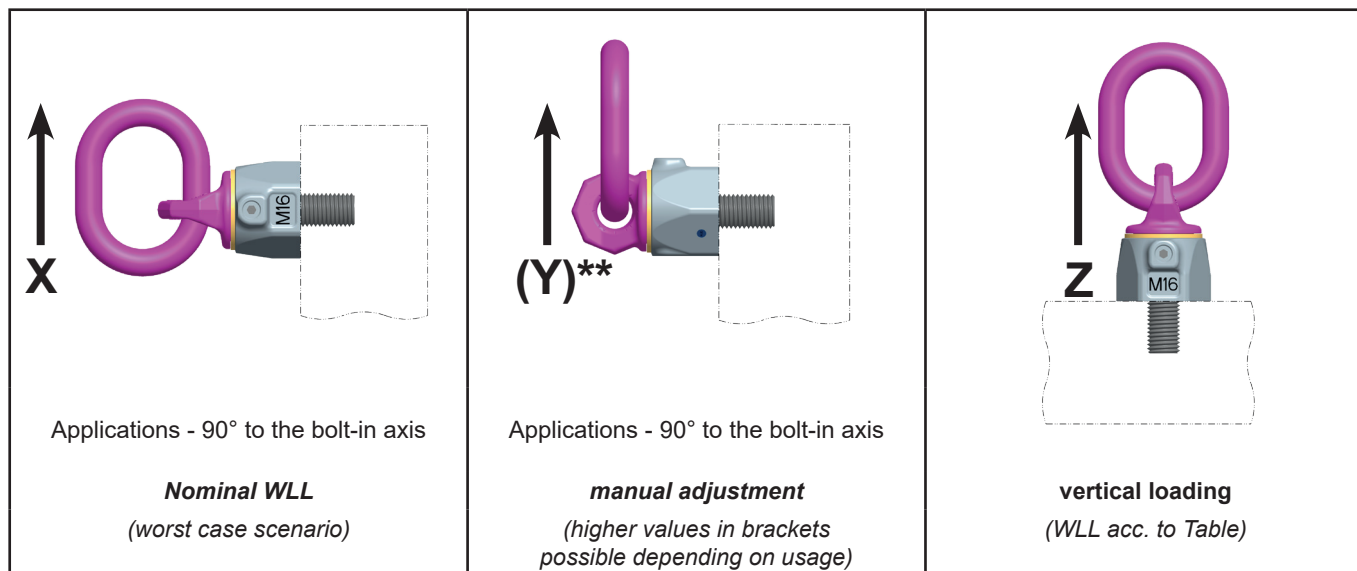
Pic. 9: Loading directions
