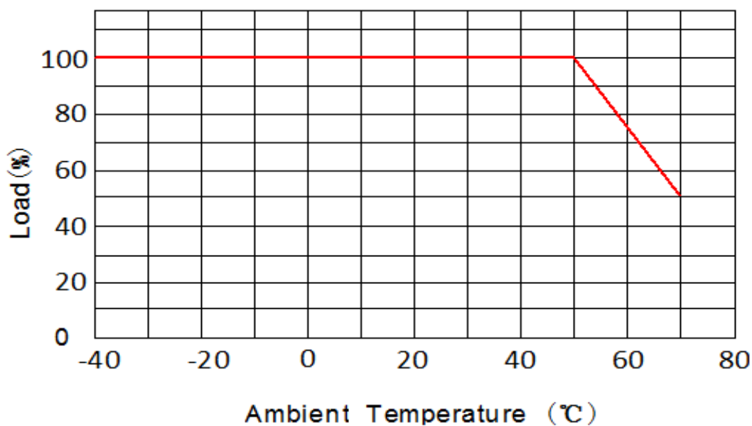
Derating Curve
