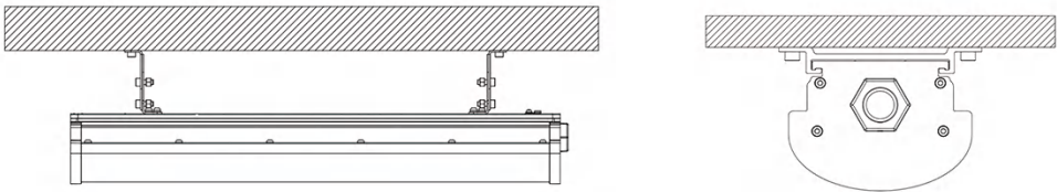
A.Ceiling mounting
