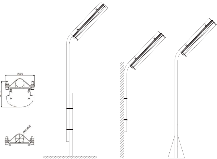
E.Pole Mounting
