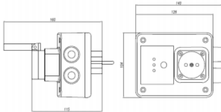
SAFEMATIC S
