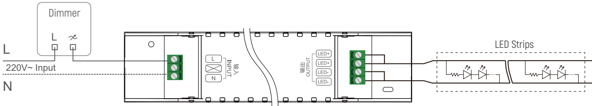
Wiring Diagram
