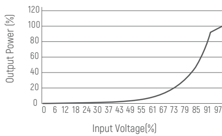
Dimming Curve
