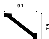
WT2 WALLSTYL® 75 x 91 x 2000 mm
