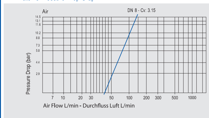
Flow Rate vs Pressure Drop Graph
