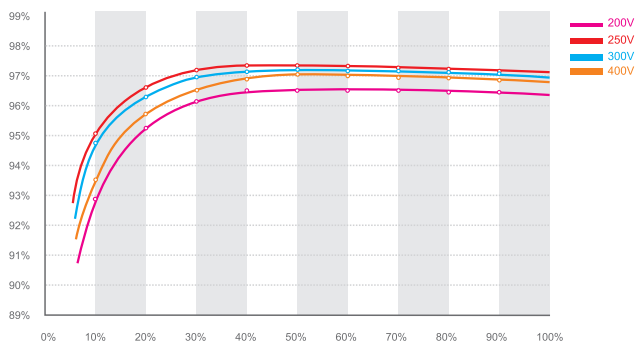
Growatt 3000-S efficiency
