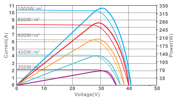
I-V characteristics at different irradiances
