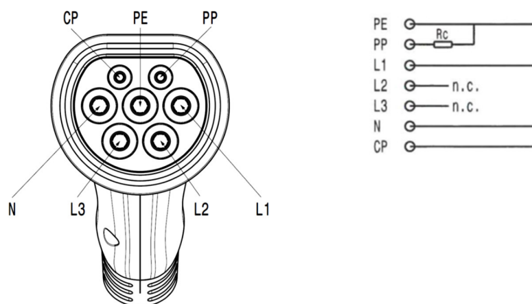
Pin assignment of the female vehicle connector
