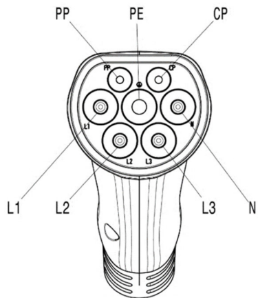
Pin assignment of the male vehicle connector
