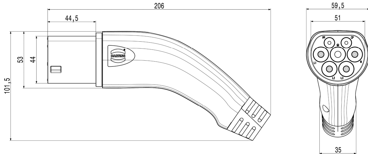
Dimensional drawing male vehicle connector
